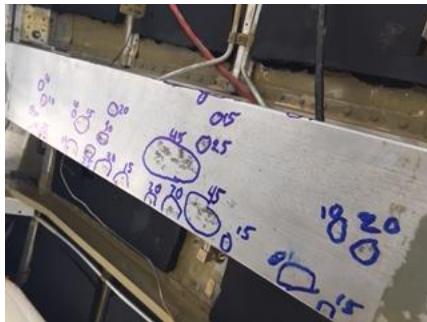
Carry-Thru-Spar Eddy Current Indications of corrosion marked
